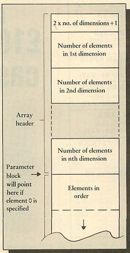
Figure 4. Format of array header
